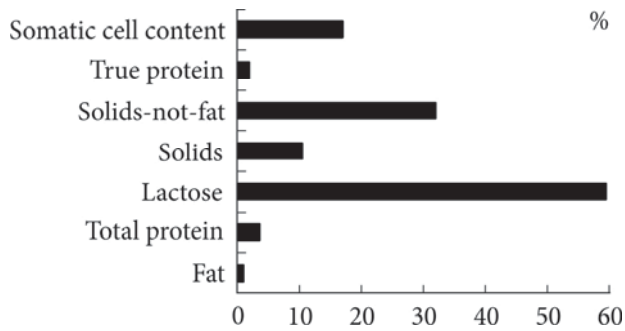
Fig. 1. Influence of content of main components of milk on its freezing point
